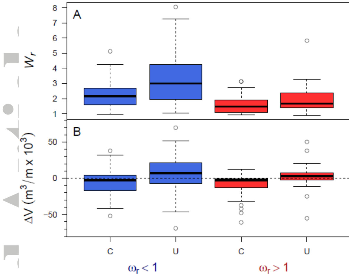
Figure 6. Boxplots comparing widening ratios (A) as well as net volume change normalized by reach length (B) among unit stream power gradient ratio and channel confinement categories: confined, C, and unconfined, U. Negative stream power gradient ( \omega_r < 1 ) results in larger and greater variability in W_r values. Median values of volume change are negative for confined and positive for unconfined reaches. Within these categories, reaches with negative stream power gradient tend to have higher median values.
