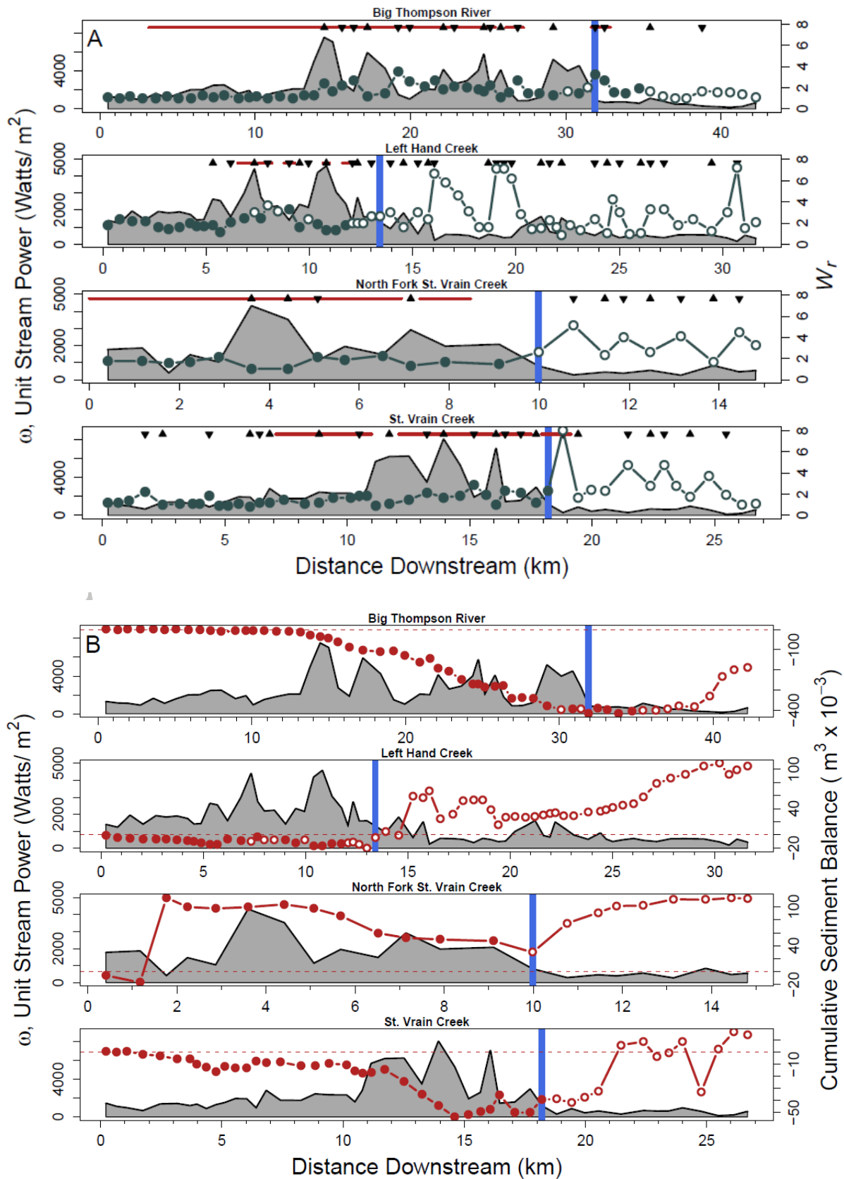
Figure 3. A: Reach scale widening ratio (green lines) plotted over the longitudinal pattern of \omega (grey polygons). Open circles indicate unconfined reaches (confinement ratio \geq 3 ) and closed circles indicate confined reaches (confinement ratio < 3 ). Vertical blue line indicates downstream-most extent of confined foothills reaches and transition to plains. Upward-facing
