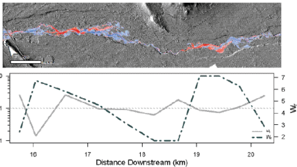
Figure 4. Image of stream segment on LH showing DEM-of-difference as well as fluvial disturbance width (top). Reach-scale pattern of W_r overlaying longitudinal pattern of \omega_r shows an oscillating expansion and contraction of W_r along LH in the plains (bottom). Peaks in \omega_r roughly align with areas of greater W_r values and troughs with smaller W_r values.
