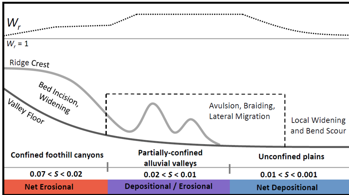
Figure 8. Conceptual figure showing downstream pattern of channel slope, confinement, and generalized geomorphic response to floods (channel width and sediment flux) within transition from foothills to plains after Bull (1988). Slope ranges will vary according to regional geology and unit peak discharge ( \text{m}^3 \text{s}^{-1} \text{km}^{-2} ) (c.f., Flores et al., 2006; Hack, 1957).
